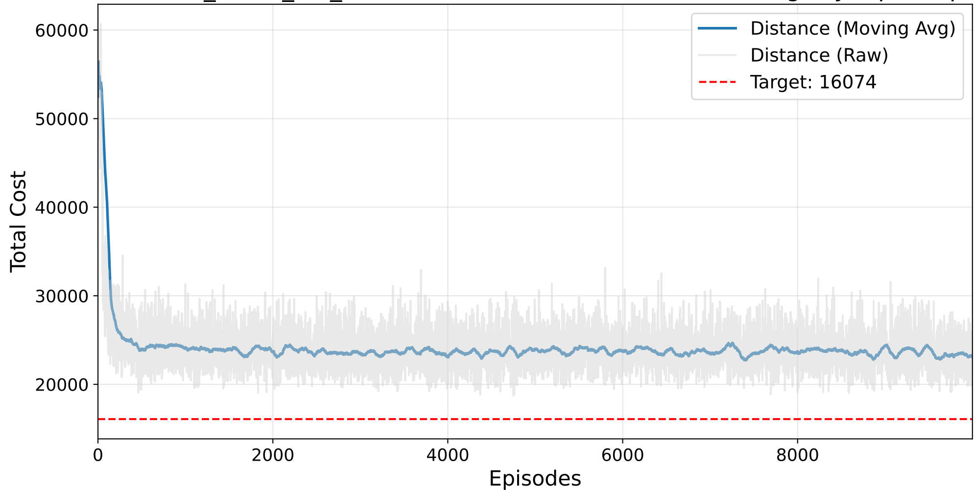
Final NO_MASK_NO_BAYESIAN Masked AutoRL-SOP Training - ry48p.2.sop
